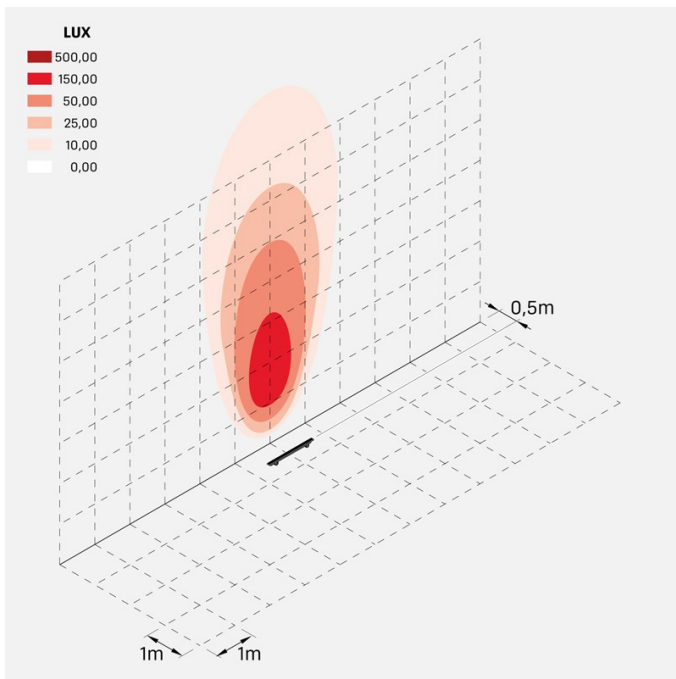
rol_1200_66W_optic_S
