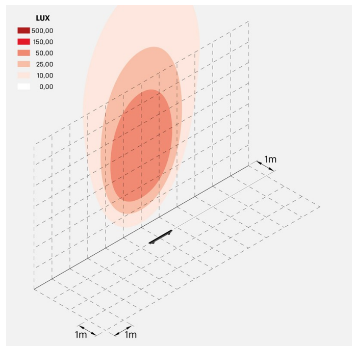
rol_1200_66W_optic_W
