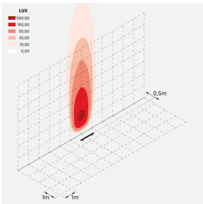
rol_1200_66W_optic_E
