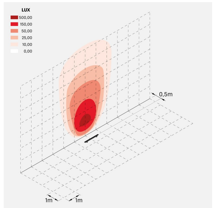
rol_1200_66W_optic_M
