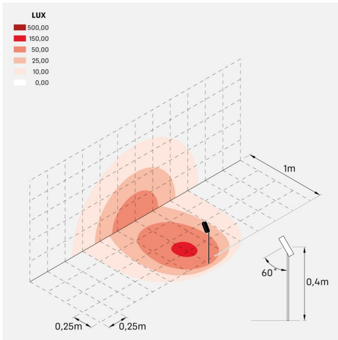
cnc_oval_garden_40_optic_D
