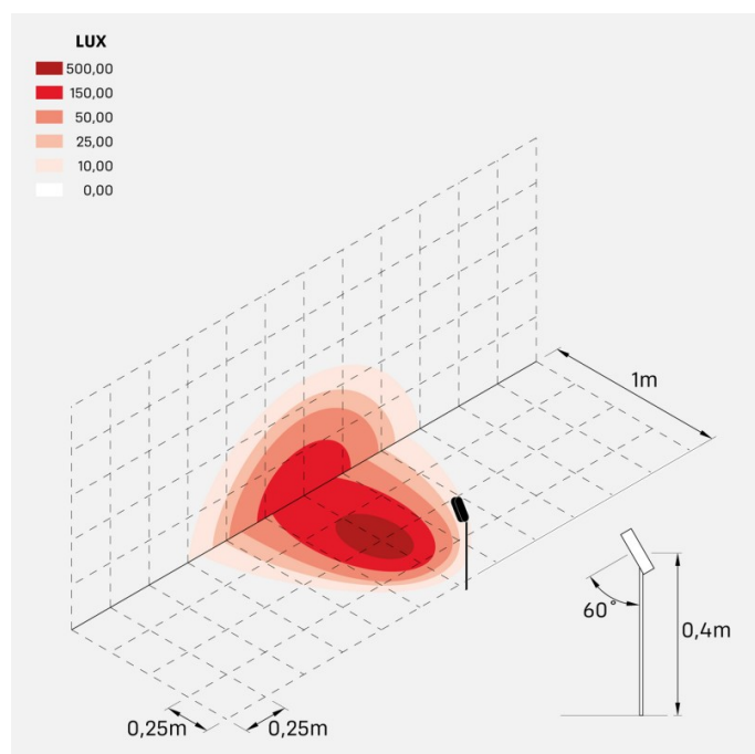
cnc_oval_garden_40_honeycomb_optic_S
