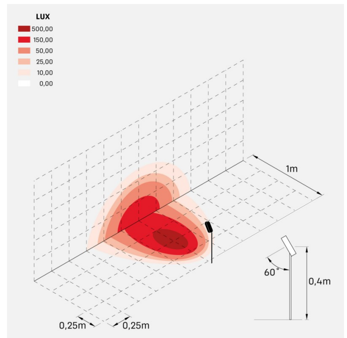
cnc_oval_garden_40_optic_S
