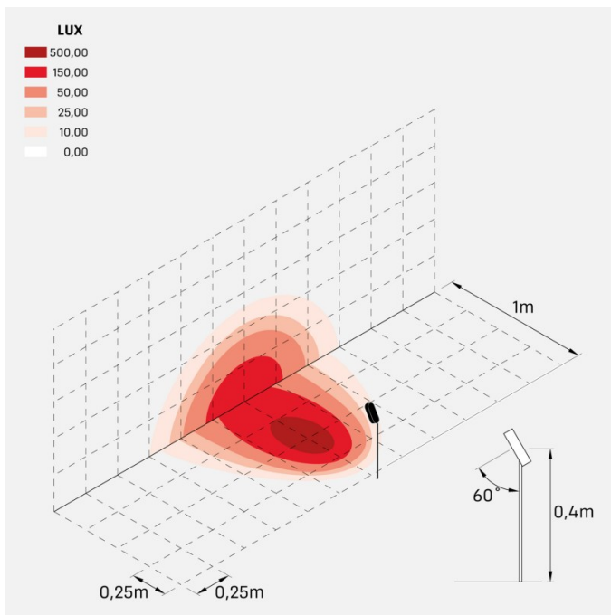
cnc_oval_garden_40_optic_M
