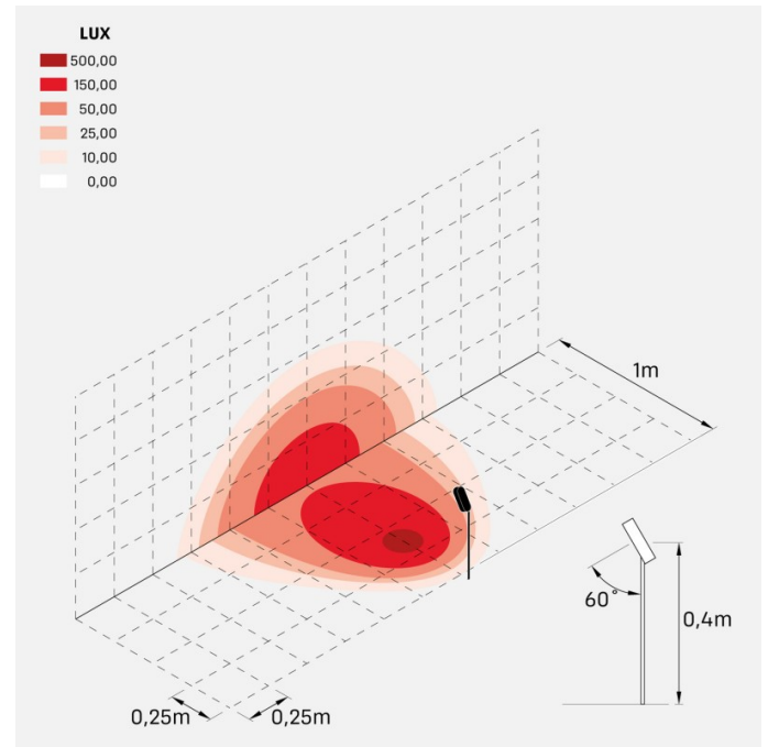
cnc_oval_garden_40_optic_L
