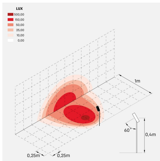
cnc_oval_garden_40_honeycomb_optic_M
