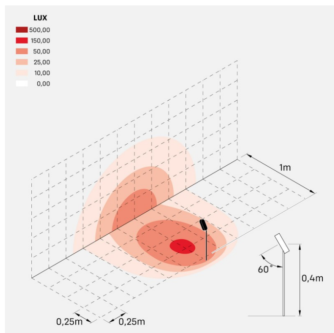
cnc_oval_garden_40_honeycomb_optic_L
