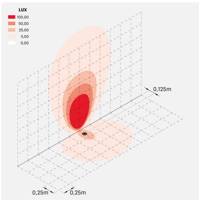
cnc_50t_20_honeycomb_optic_L
