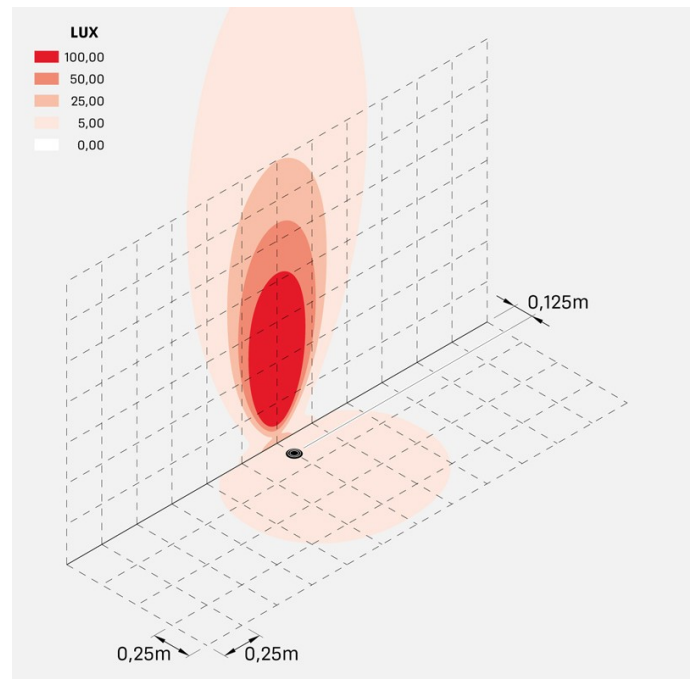
cnc_50t_20_honeycomb_optic_M
