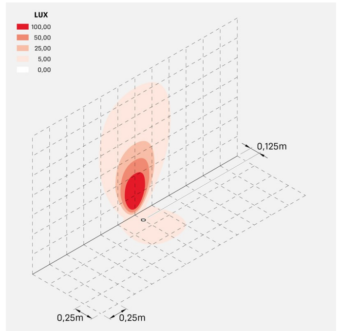
cnc_35t_simm_20_trimless_optic_L
