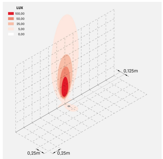
cnc_35t_simm_20_trimless_optic_S
