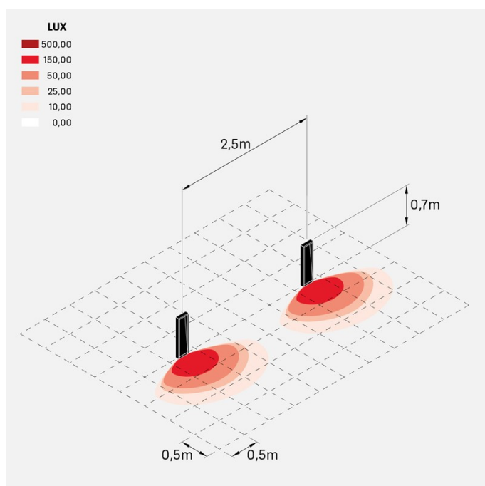
arke700_full_220v
