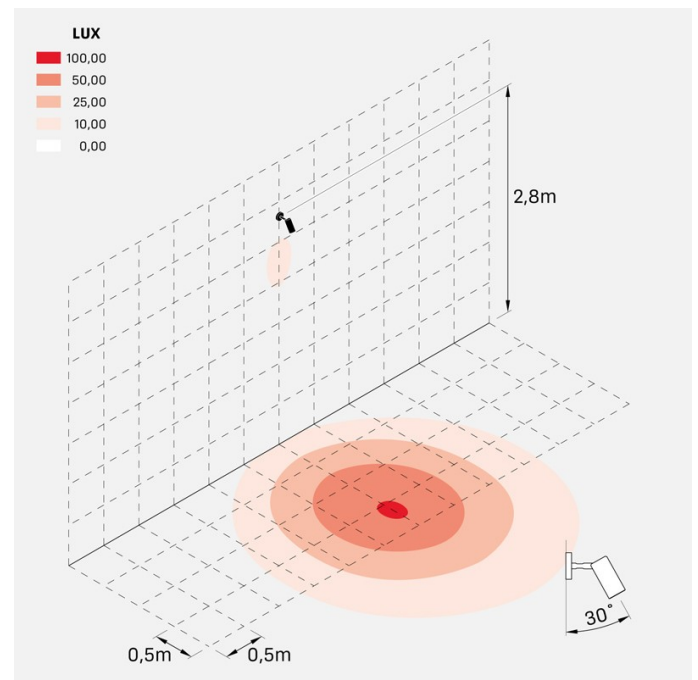
ago_wall_power_optic_S
