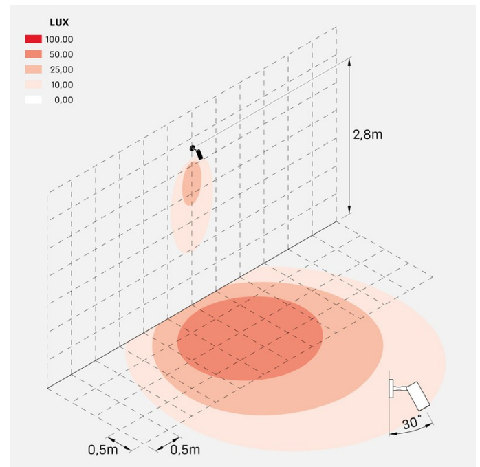
ago_wall_power_optic_L
