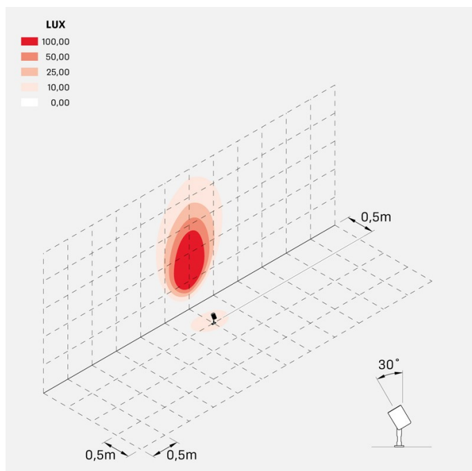
ago_garden_honeycomb_optic_S
