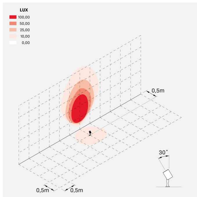
ago_garden_honeycomb_optic_M
