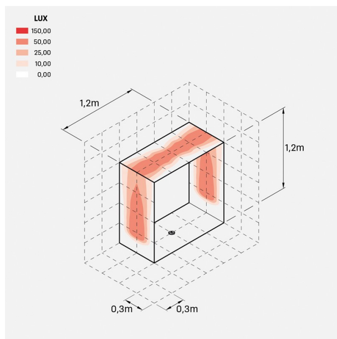
trim_cnc_finestra120x120
